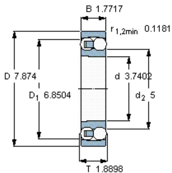
圆锥孔，圆锥 1: 12
